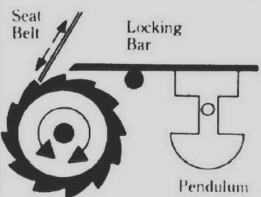
Ratchet Mechanism
