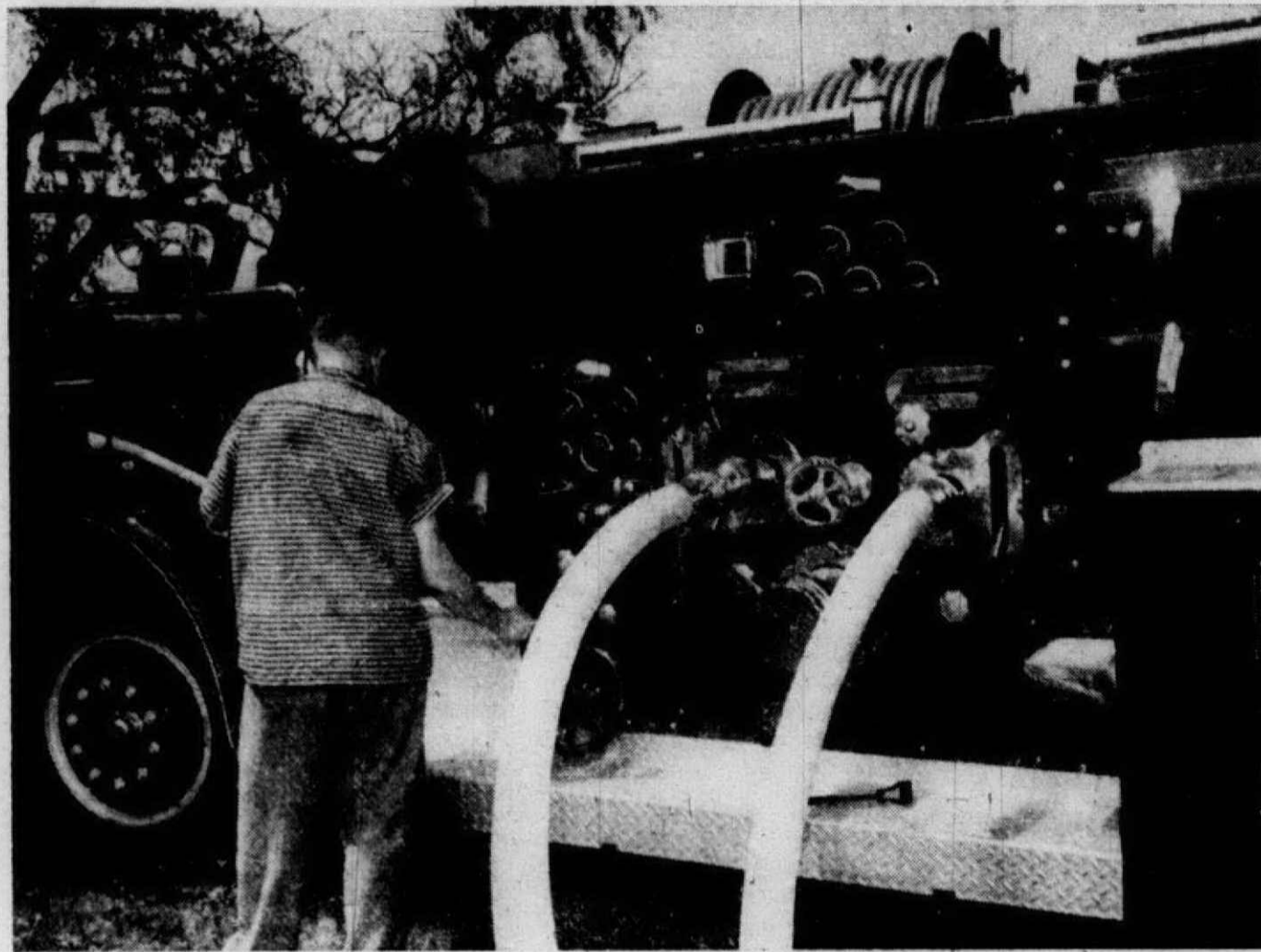
LOTS OF DIALS, valves and hose connections make a complicated looking picture of the city's new fire engine. A company engineer is shown at work during the three-hour test last week at Wilcox Lake. Rated at 1,000 gallons a minute, the pumper once hit 1,136 gallons.
